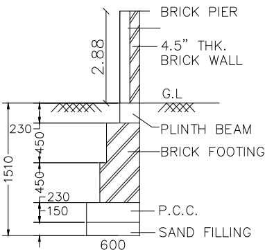
COMPOUND WALL DETAILS
