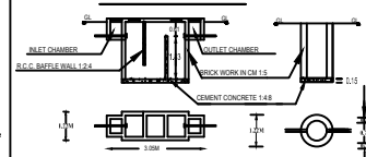
DETAILS OF SEPTIC TANK & SOAK PIT.
