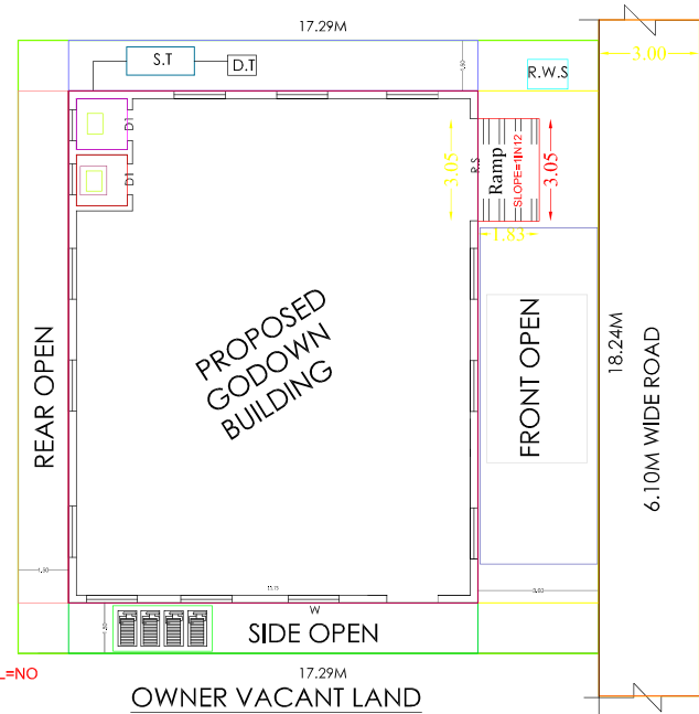
DETAILED SITE PLAN SCALE 1:100
