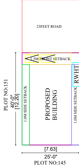
SITE PLAN SCALE :1:100
