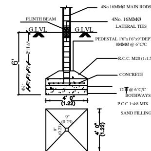
FOUNDATION DETAIL
