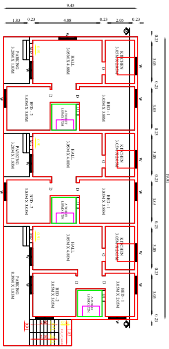
PROPOSED GROUND FLOOR PLAN
