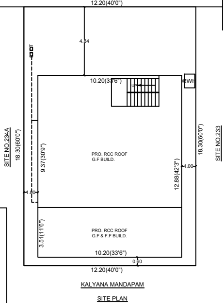
SITE PLAN
