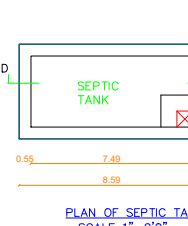
PLAN OF SEPTIC TANK SCALE 1" = 6'0"
