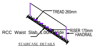
STAIRCASE DETAILS
