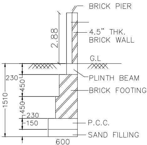
COMPOUND WALL DETAILS
