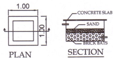
RAIN WATER HARVESTING TANK
