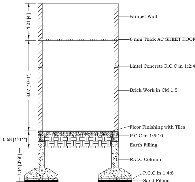
SECTION X-X
