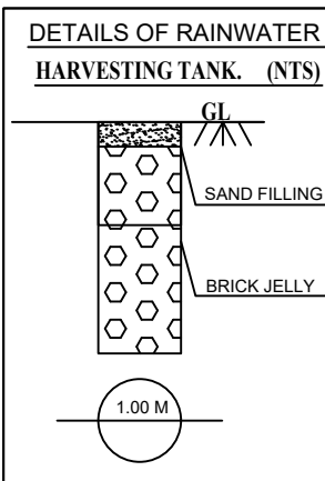
DETAILS OF RAINWATER HARVESTING TANK. (NTS)
