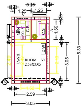
PRO. GROUND FLOOR SHOP PLAN
