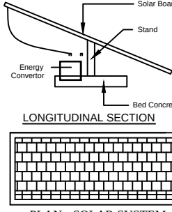
PLAN SOLAR SYSTEM Not To Scale
