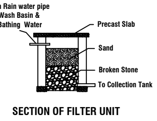
SECTION OF FILTER UNIT
