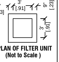
PLAN OF FILTER UNIT (Not to Scale)
