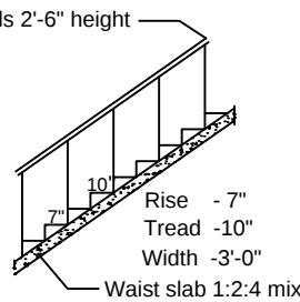
Handrails 2'-6" height
