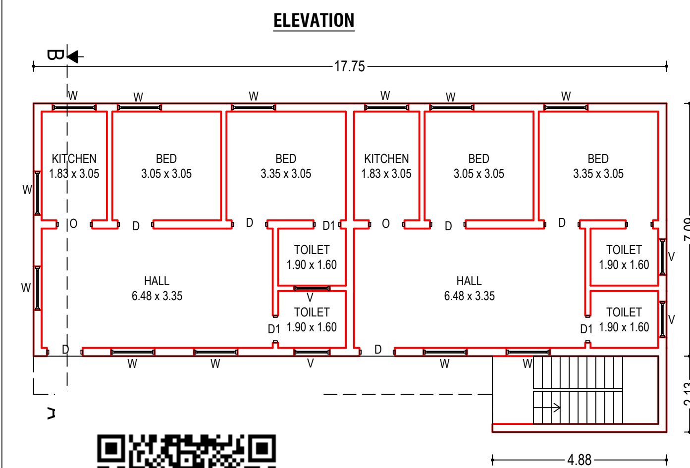
VD FLOOR PLAN
