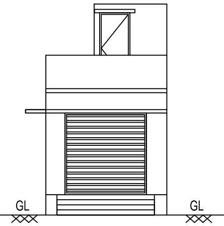
ELEVATION (WEST FACING)
