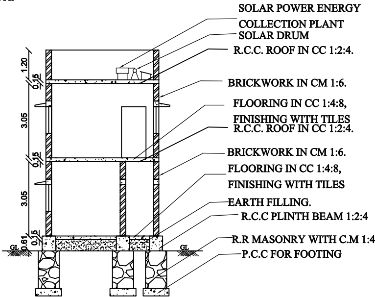
CROSS SECTION ON 'AB' & 'CD'
