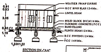
SECTION ON-AA'
