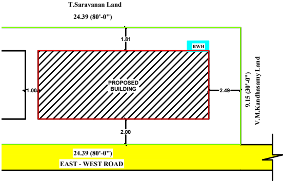
SITE TAKEN PLAN (scale - 1:200)
