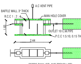
SEPTIC TANK (ST) AND TRENCH (DT)
