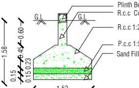
COLUMN FOOTING DETAILS
