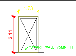
WICKET GATE
