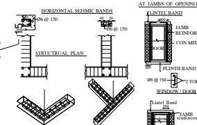
HORIZONTAL SEISMIC BANDS
