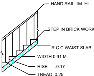
STAIR DETAIL
