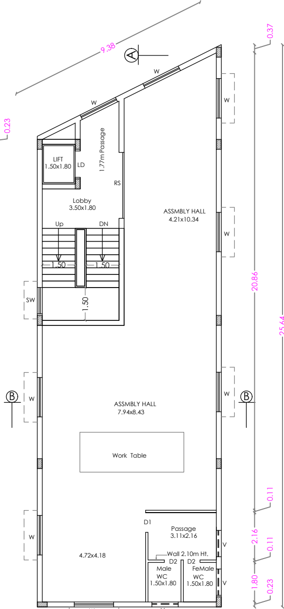
TYPICAL FLOOR PLAN
