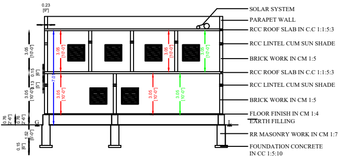
SECTION "AA","BB"
