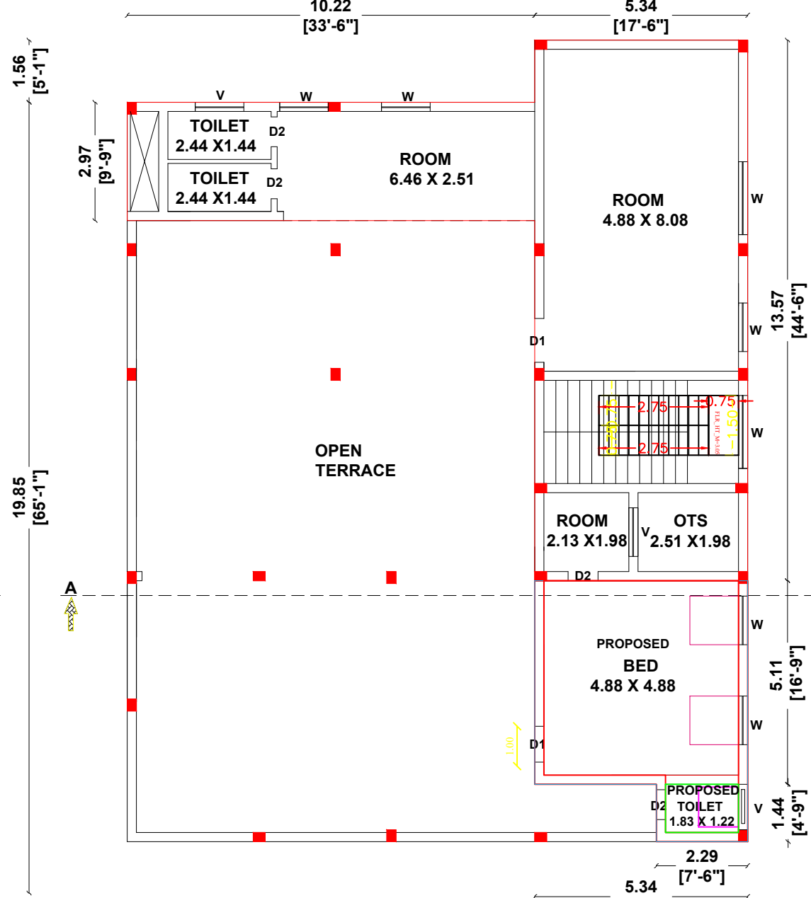
EXISTING & PROPOSED SECOND FLOOR PLAN
