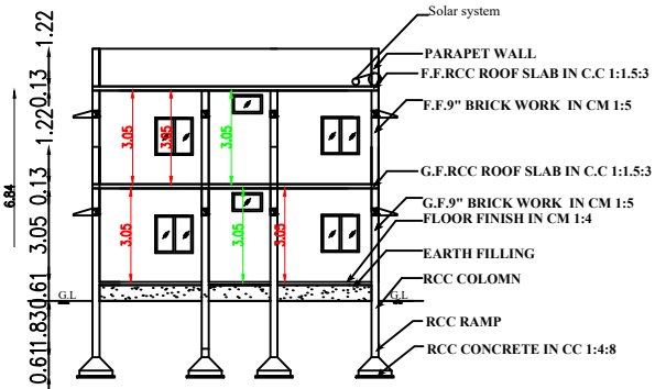
SECTION ON - AA & BB
