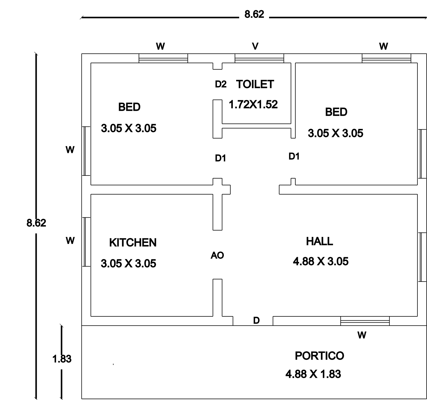
EX.GROUND FLOOR PLAN
