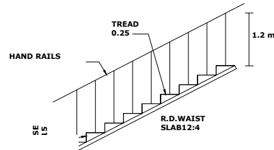
AIRCASE DETAILS
