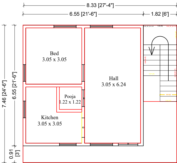
Building Plan Ground Floor
