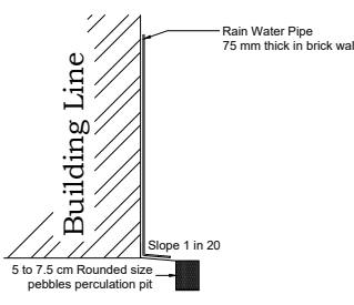
RAINWATER HARVESTING
