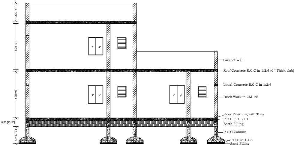
SECTION X-X
