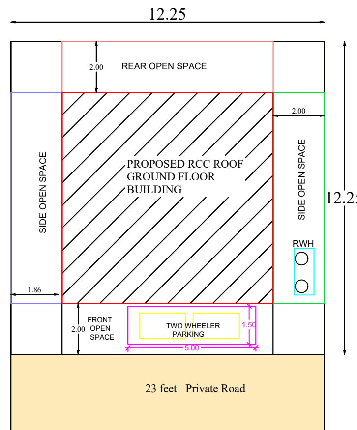
SITE & LOCATION PLAN SCALE - 1: 100
