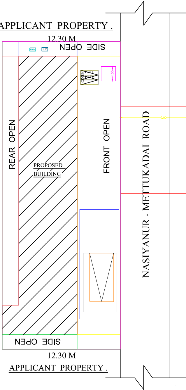
SITE PLAN (TAKEN AREA) SCALE 1:100
