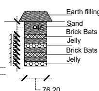
SECTION ON B-B.
