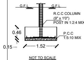
COLUMN POST DETAILS
