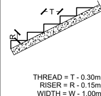
STAIRCASE DETAILS
