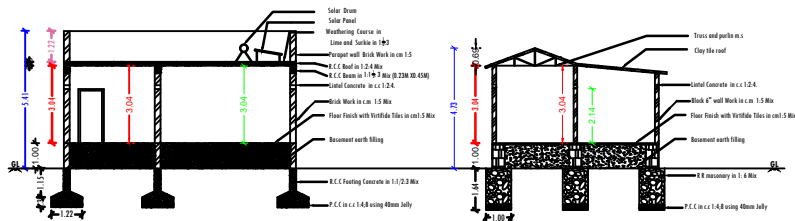
SECTION ON "BC"
