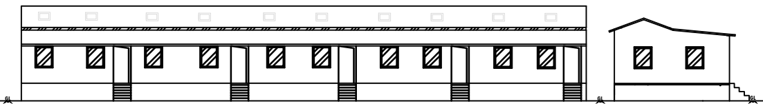
ELEVATION ON "A"
