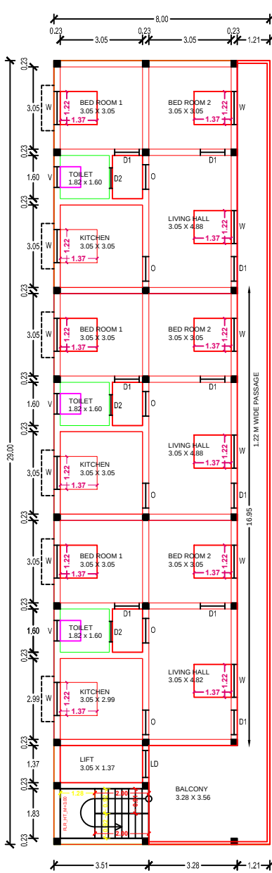
STILT FLOOR PLAN ( BLOCK - 1 - PROPOSED RESIDENTIAL BUILDING ) FIRST FLOOR PLAN ( BLOCK - 1 - PROPOSED RESIDENTIAL BUILDING ) SECOND FLOOR PLAN ( BLOCK - 1 - PROPOSED RESIDENTIAL BUILDING ) THIRD FLOOR PLAN ( BLOCK - 1 - PROPOSED RESIDENTIAL BUILDING )
