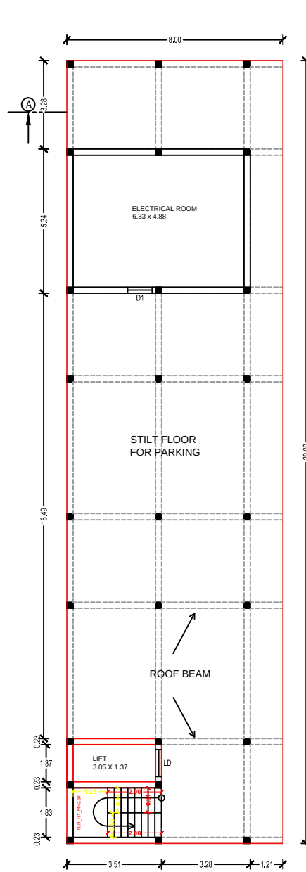
STILT FLOOR PLAN ( BLOCK - 1 - PROPOSED RESIDENTIAL BUILDING ) FIRST FLOOR PLAN ( BLOCK - 1 - PROPOSED RESIDENTIAL BUILDING ) SECOND FLOOR PLAN ( BLOCK - 1 - PROPOSED RESIDENTIAL BUILDING ) THIRD FLOOR PLAN ( BLOCK - 1 - PROPOSED RESIDENTIAL BUILDING )
