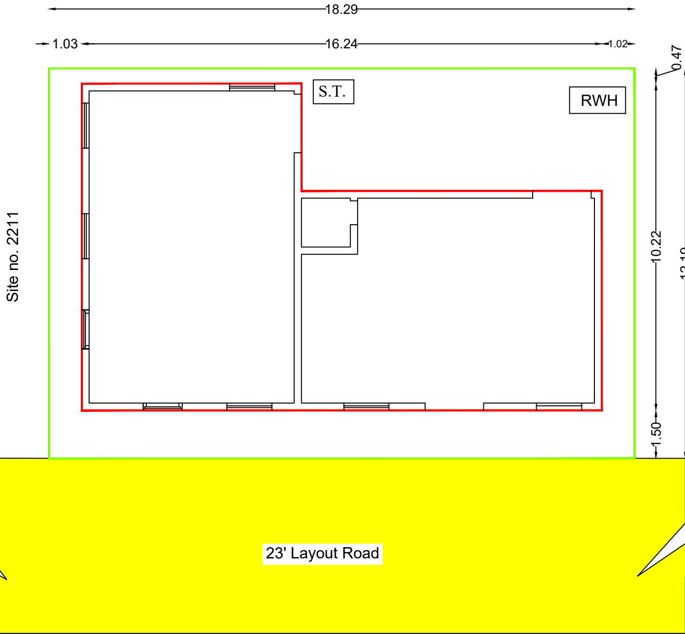
SITE PLAN
