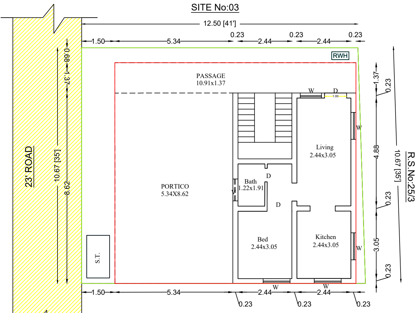
K.SEKAR PROPERTY GROUND FLOOR & SITE PLAN
