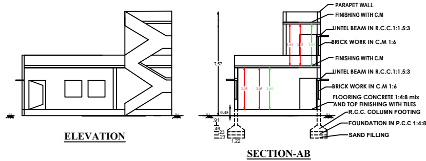
SECTION-AB
