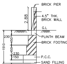
COMPOUND WALL DETAILS
