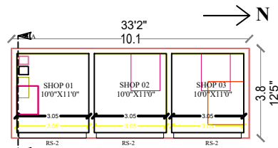
GROUND FLOOR RCC PLAN
