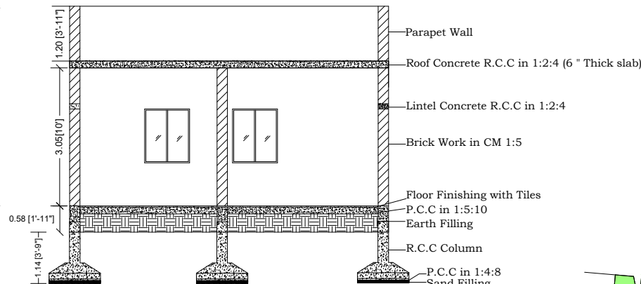
SECTION X-X
