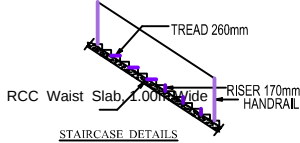
STAIRCASE DETAILS
