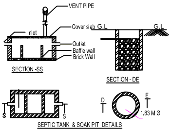
SEPTIC TANK & SOAK PIT DETAILS
