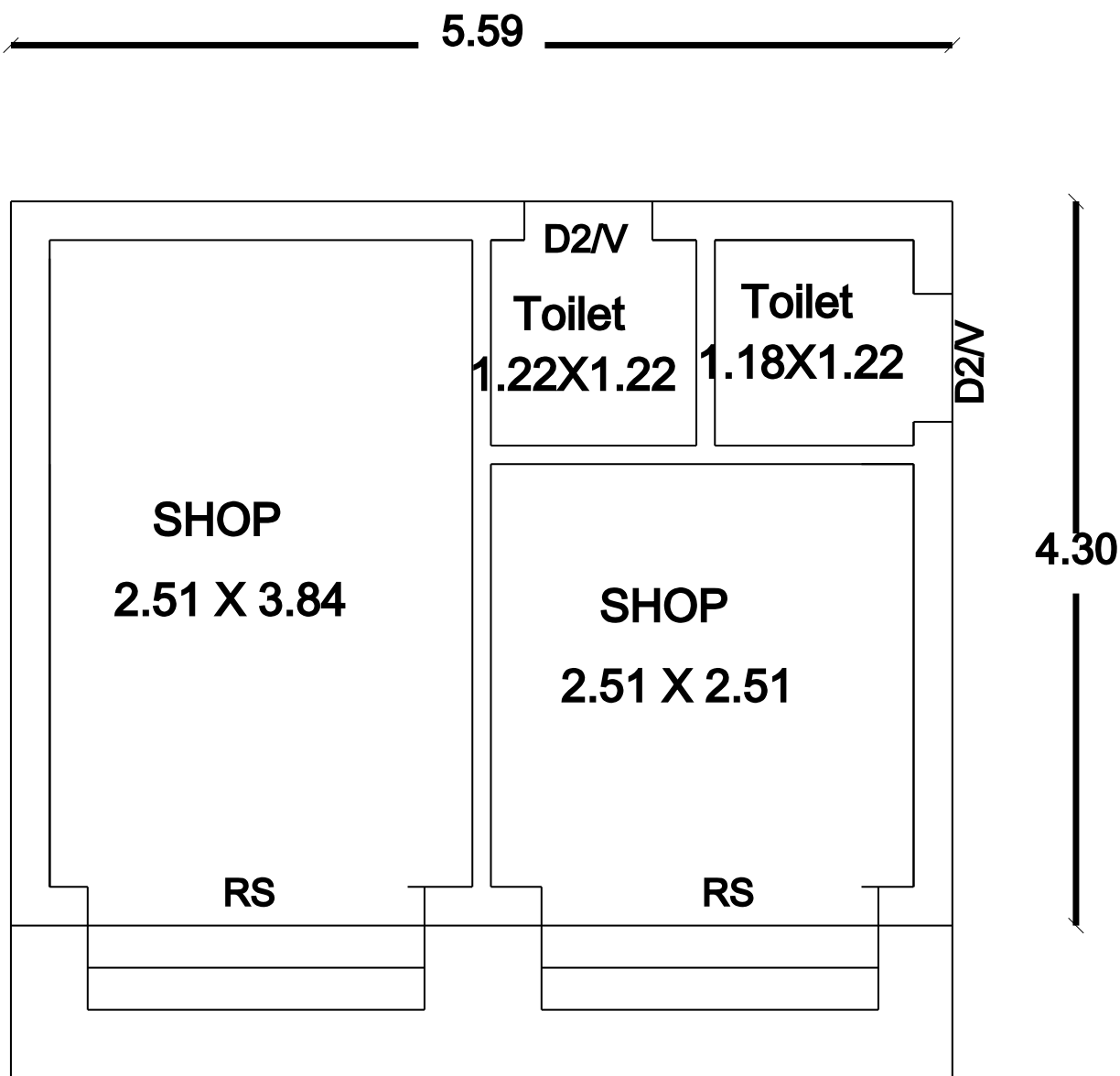
PLAN
