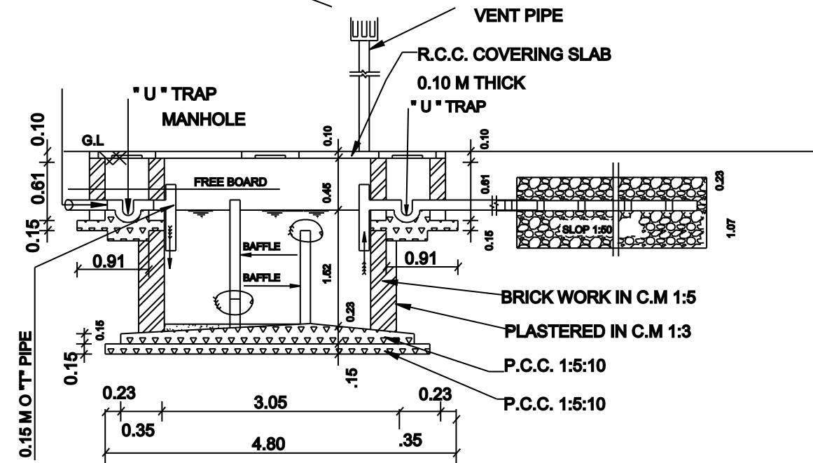
LONGITUDINAL SECTION IN "XX"
