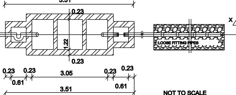
SEPTIC TANK & DISPERSION TRINCH
