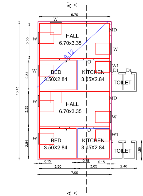
GROUND FLOOR TERRACE FLOOR
