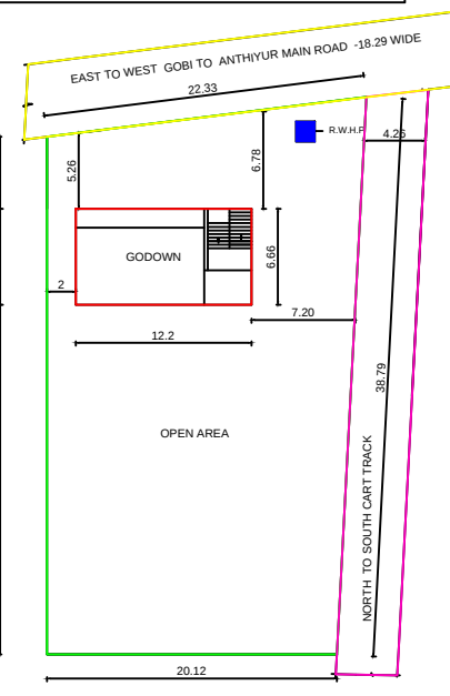
SITE PLAN
