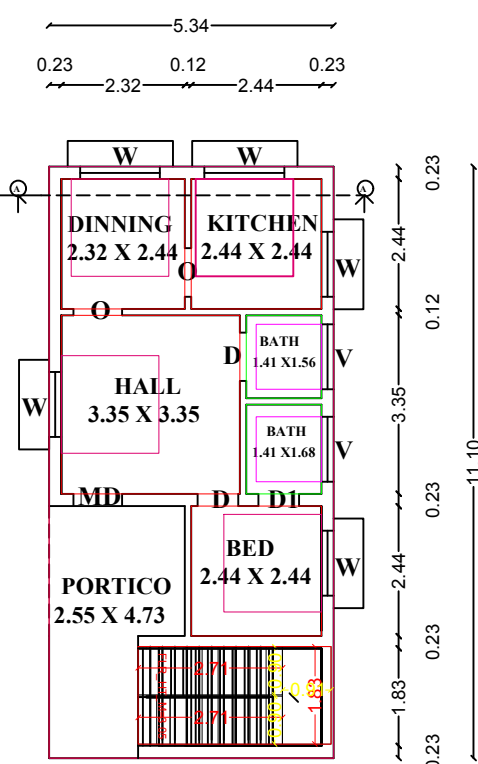
PRO. GROUND FLOOR
