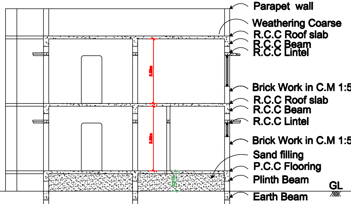
SECTION ON "RR"
