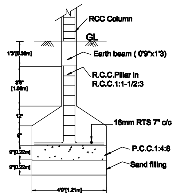
FOUNDATION DETAILS
