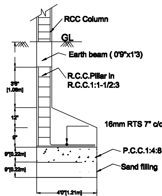
FOUNDATION DETAILS
