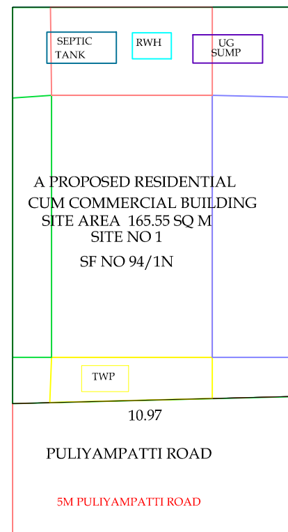
SITE PLAN
