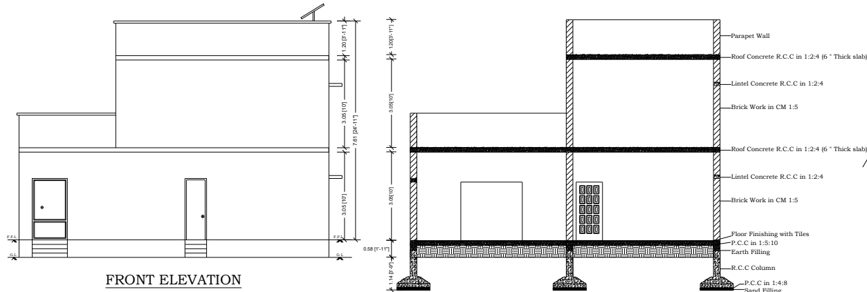
SECTION X-X
