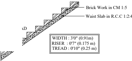
STAIRCASE DETAILS
